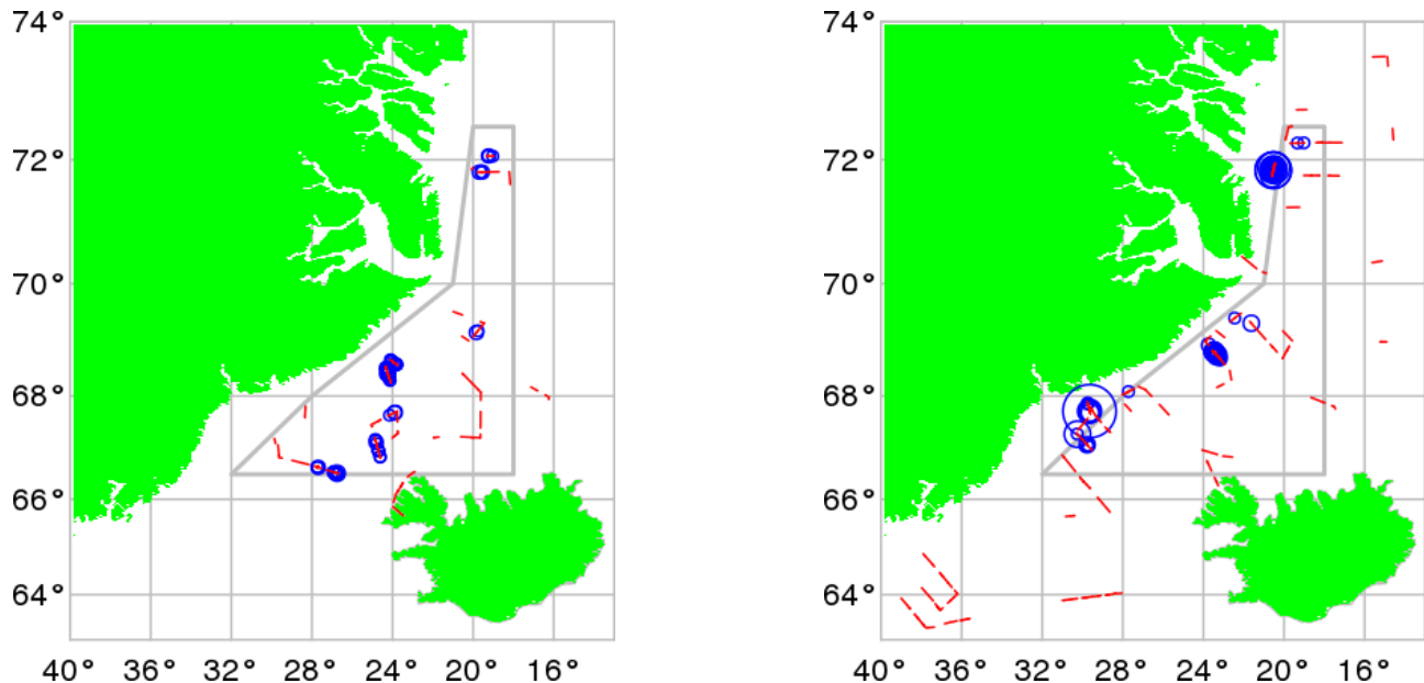
Fig 1. Sightings of humpback whales (blue) and covered track lines (red) in capelin surveys Sept-October 2015 (left) and 2016 (right). Estimates have been produced for 2015 (grey bordered area).
