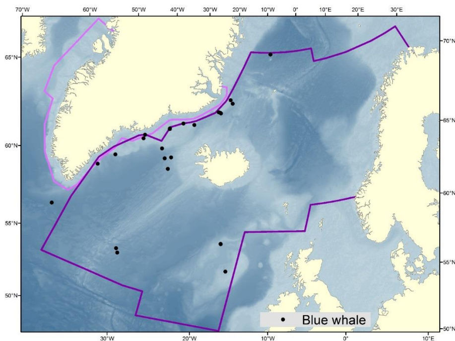
Fig. 18. Sightings of blue whales during NASS2015.
