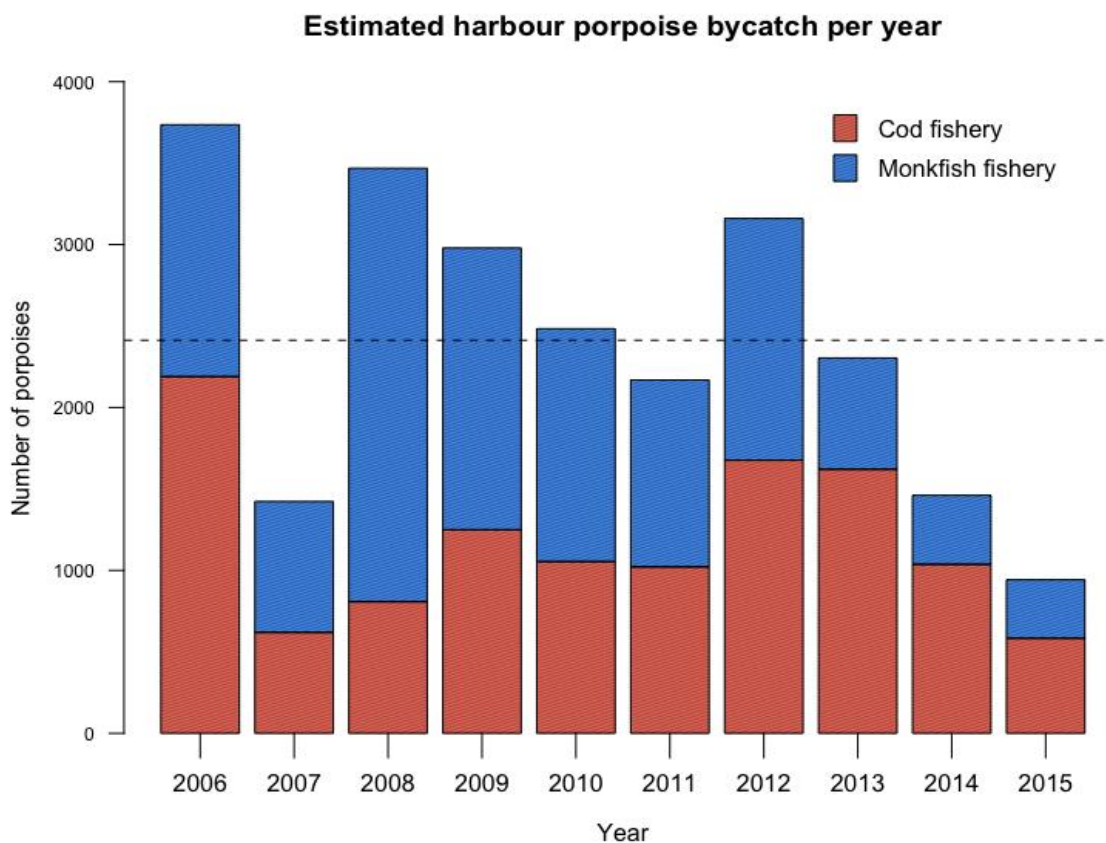
Figure 1. Estimated harbour porpoise bycatch in the Norwegian coastal gillnet fisheries targeting cod and monkfish. Estimates were derived using a stratified ratio estimator approach with data stratified by year, season and region. The dashed horizontal line represents average yearly bycatch across the ten-year period.
