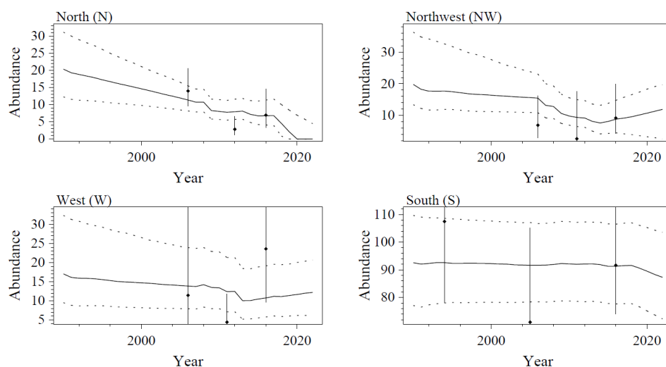
Figure 2. Projections of harbour porpoise from the agreed assessment. The solid curve is the median, the dotted lines the 90% credibility intervals, and the dots with bars the agreed abundance estimates and their 90 % confidence interval.
