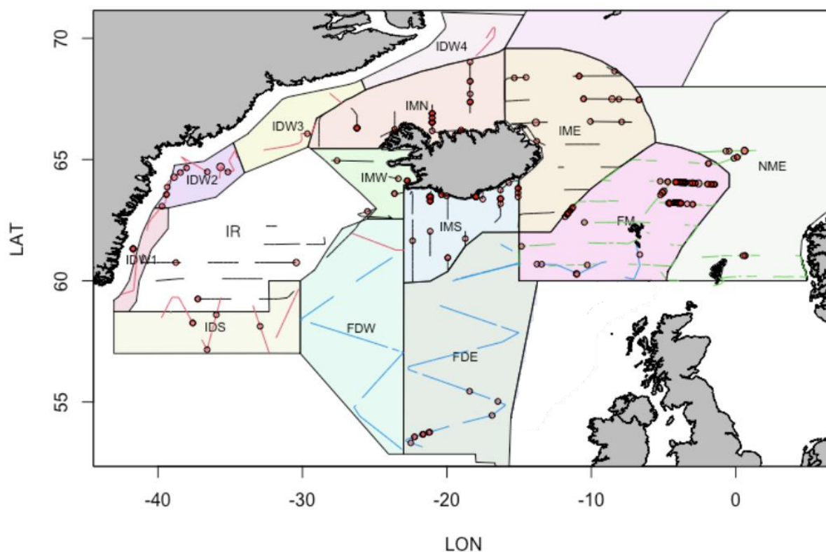
Figure 2. Realised survey effort and minke whale sightings achieved by the Faroese and Icelandic vessels.
